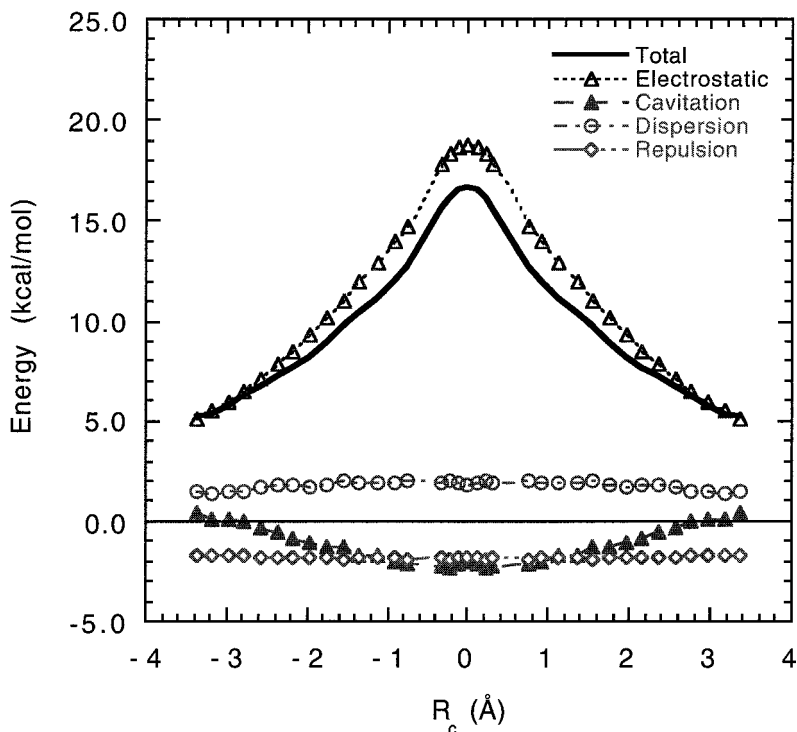
Figure 2. BH & HLYP/6-31 +G(d,p) total hydration energy (—) and its individual contributions (( \Delta ), electrostatic; ( \blacktriangle ), cavitation; ( \circ ), dispersion; ( \diamond ), repulsion) plotted as functions of the reaction coordinate R_c of the S_N2 Cl^- + CH_3Cl reaction. All contributions are relative to their separated reactant values.
