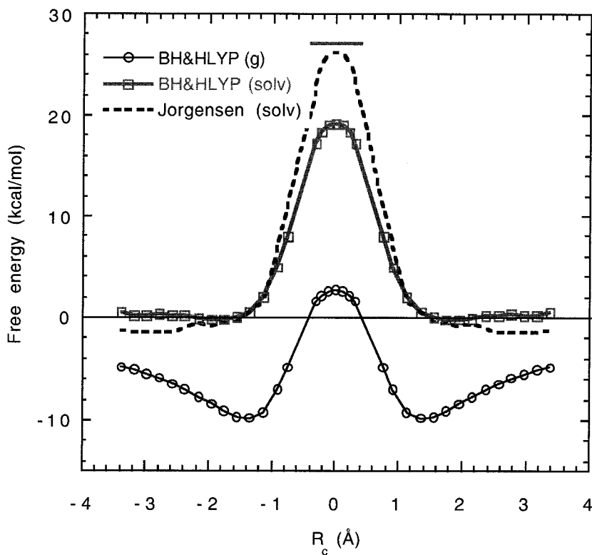
Figure 1. Reaction profiles of the S_N2 Cl^- + CH_3Cl reaction in the gas phase (potential energy) (thin solid curve) and in aqueous solution (pseudo-free energy) (thick solid curve). The solid curves are from the BH & HLYP-GCOSMO calculations using the 6-31+G(d,p) basis set, and the broken curve is from MC simulations [111]. The horizontal bar is the free energy of activation with added contribution from the solute internal degrees of freedom.
